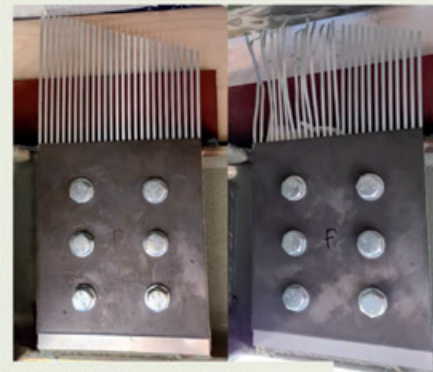
Fig. 5 Displacement device before and after the explosion
